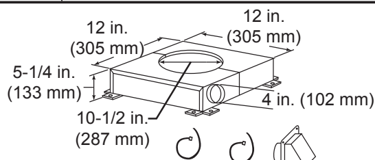
CAK4A Chimney Air Kit
