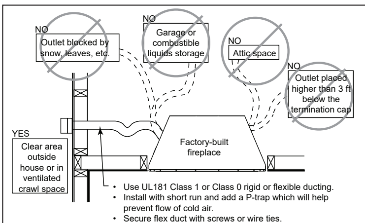
► Figure 3.8 Outside Air Installation
