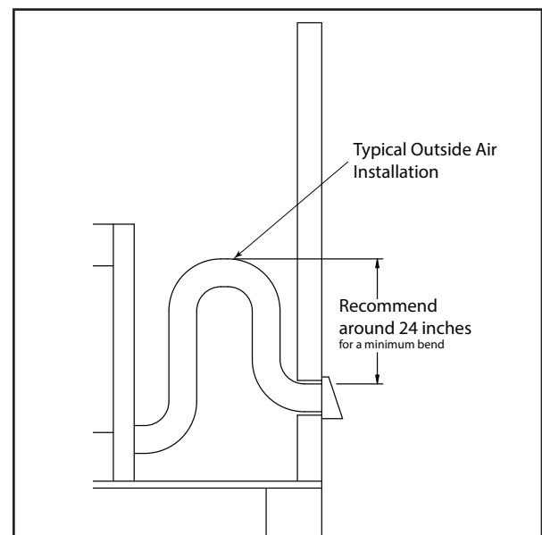
► Figure 3.10 Outside Air Installation with Cold Air Trap
