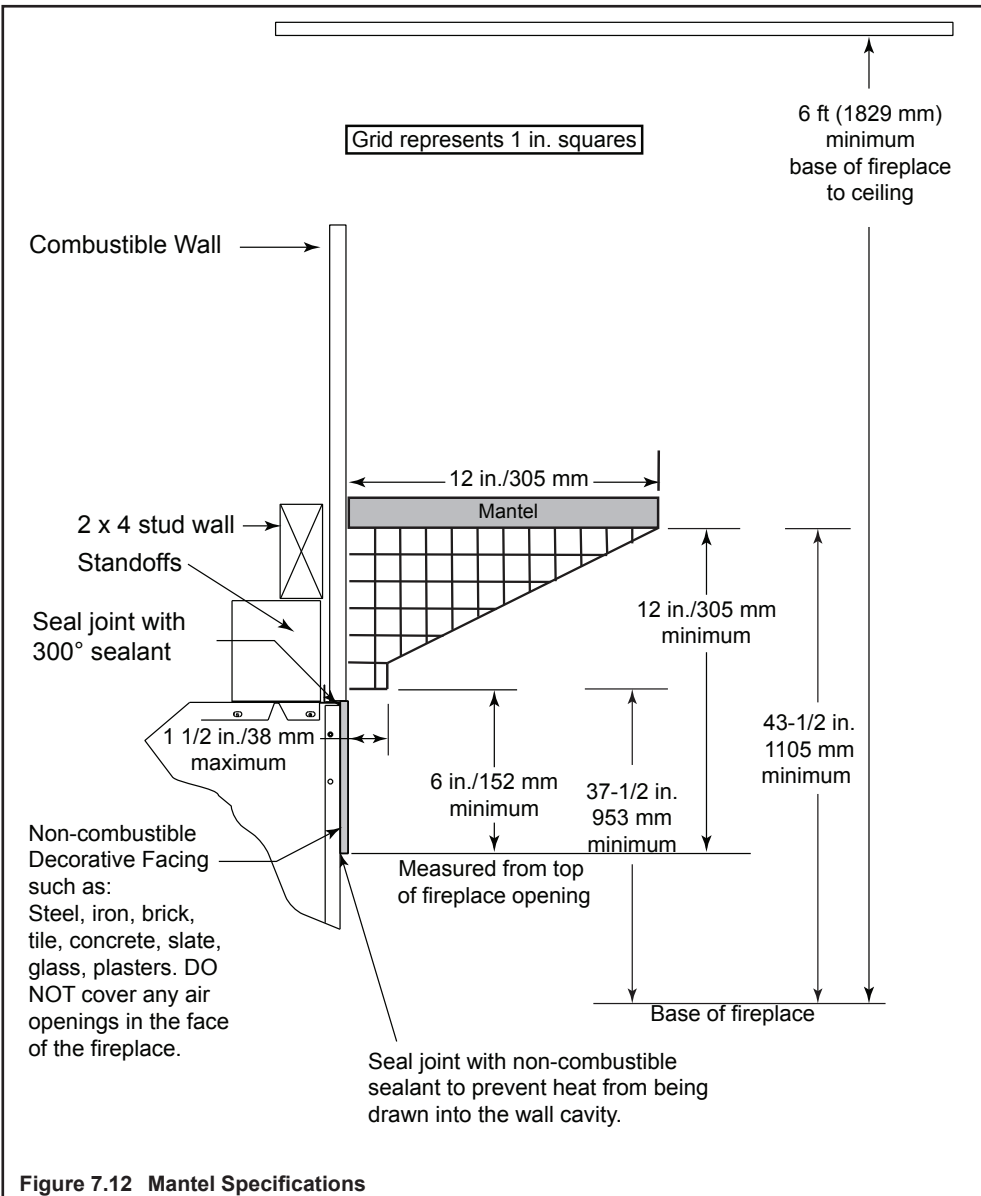
Figure 7.12 Mantel Specifications
