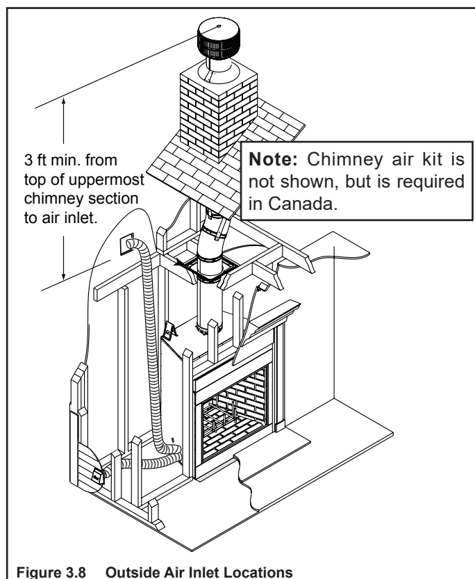
Figure 3.8 Outside Air Inlet Locations
