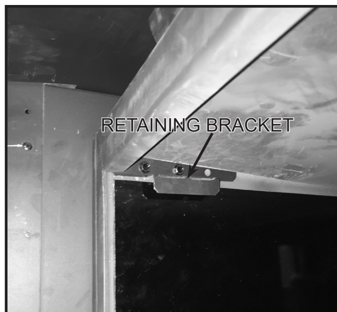
Figure 5 Retaining Bracket Installation - Side Panel
