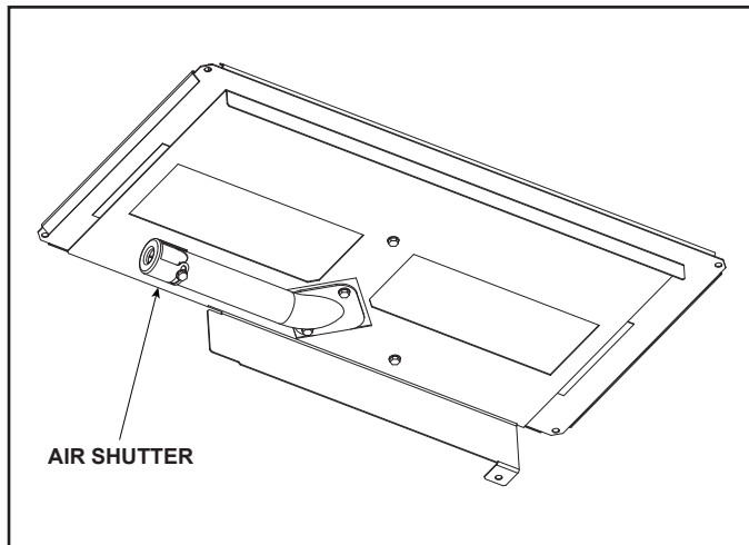
Figure 9.1 Air Shutter
