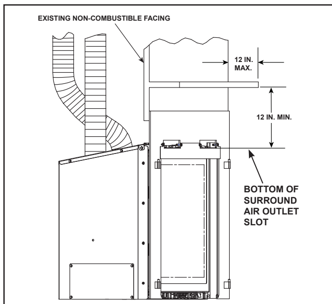
Figure 10.1 Mantel Clearance
