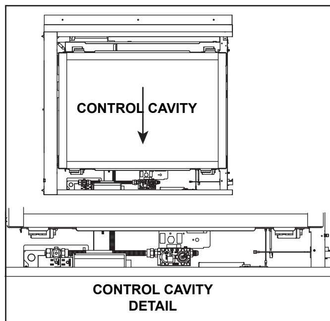
3.5 Control Cavity Location (PIER-36TRB-IFT Shown)
