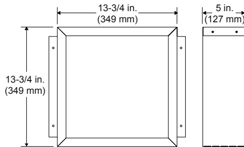
BEK Trap Cap Brick Extension
