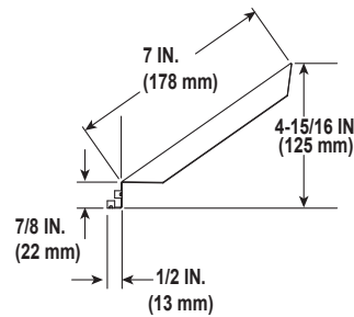
BEK Trap Cap Brick Extension
