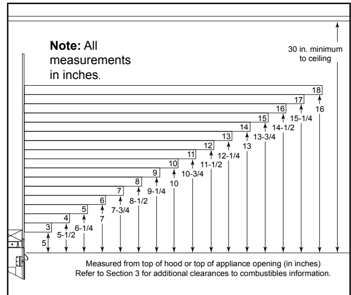
Figure 10.1 Minimum Vertical and Maximum Horizontal Dimensions
