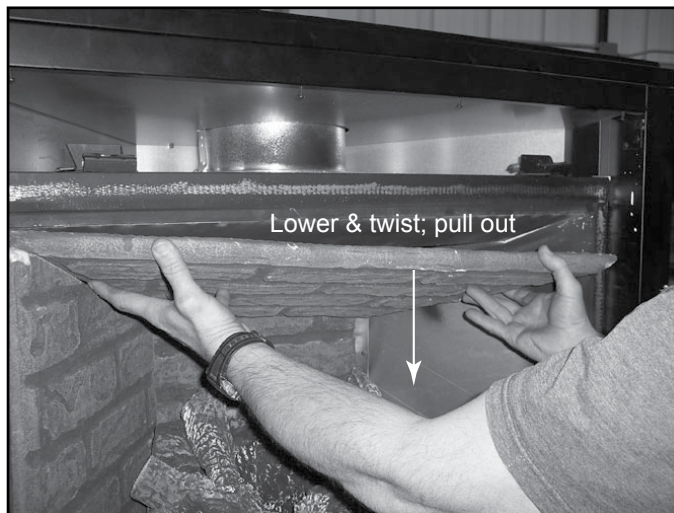
Figure 4.18 Remove Top Refractory
