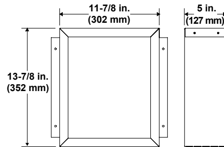
DVP-BEK2 DVP-HPC Cap Brick Extension
