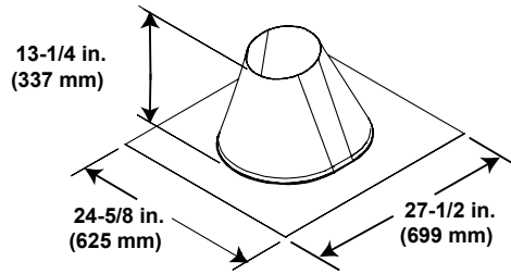
RF6 Roof Flashing
