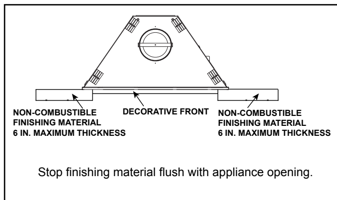
Figure 10.3 Non-Combustible Finishing Material (Sides and Top of Appliance)
