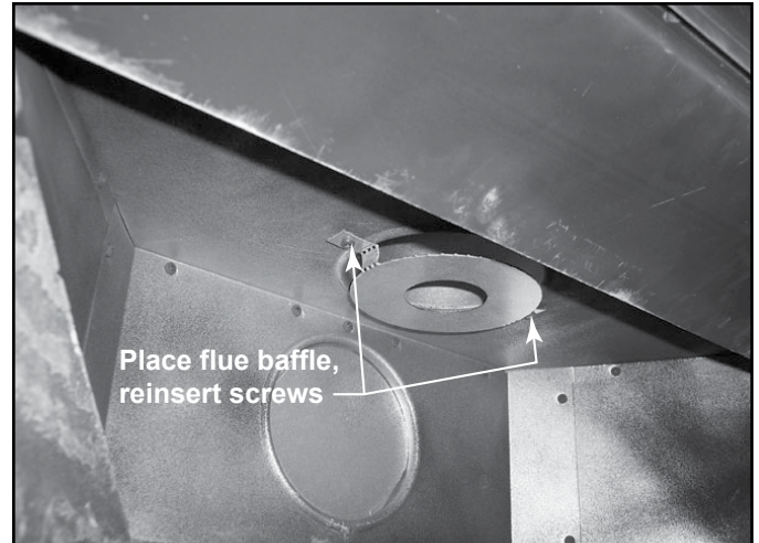
Figure 4.19 12-30 Foot Vertical Run
