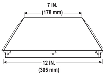
TRAP-VSS Vinyl Siding Shield
