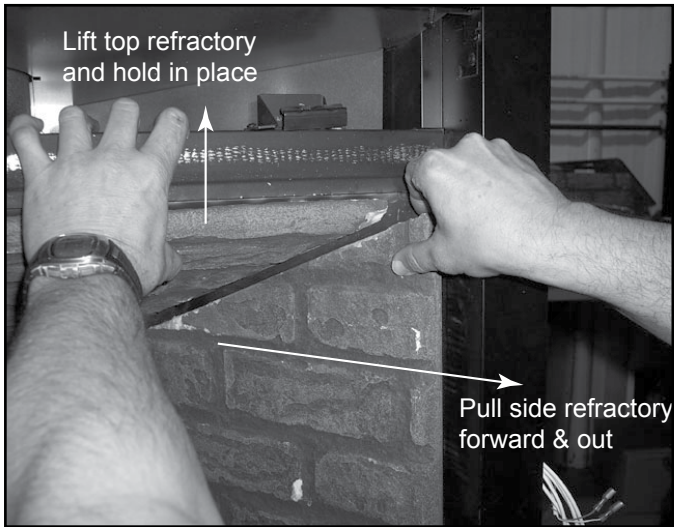
Figure 4.17 Remove Side Refractory
