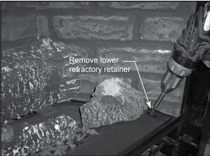
Figure 4.17 Remove Refractory Retainer
