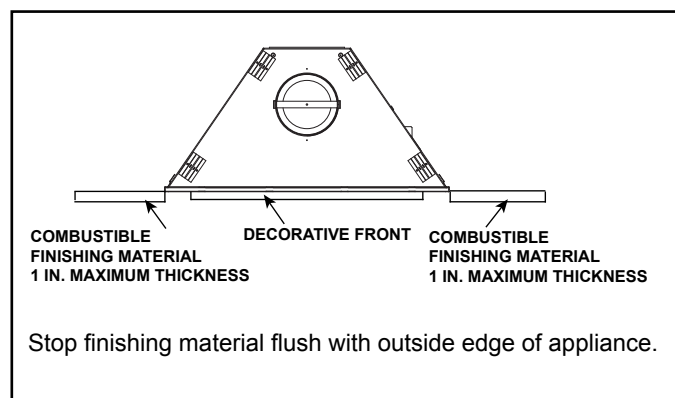
Figure 10.4 Combustible Finishing Material (Sides of appliance only. See Figure 10.1 for Combustible Mantel Clearances)
