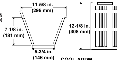
COOL-ADDM Cap Shield
