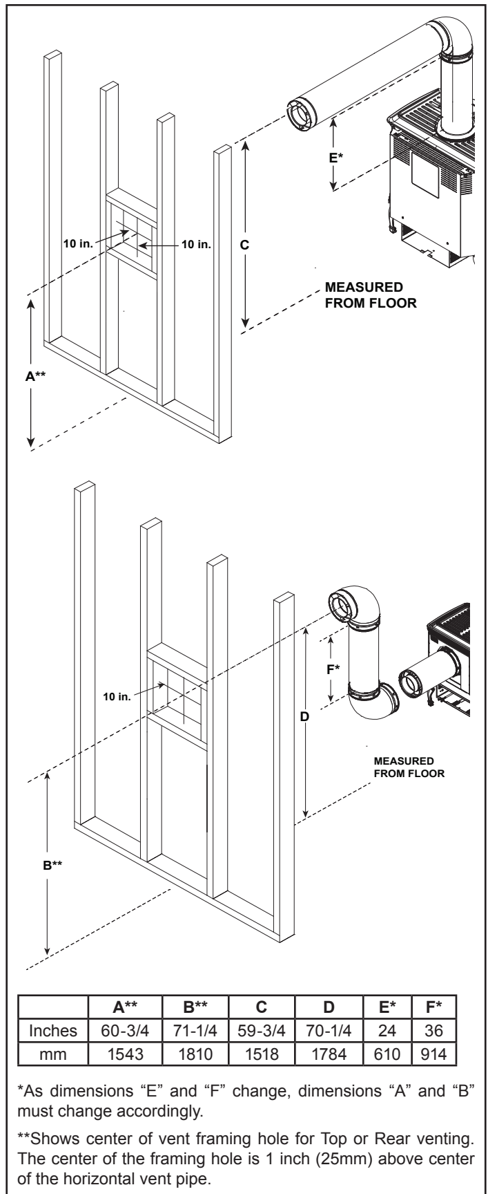
Figure 5.2 - Wall Penetration
