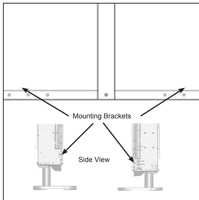
Figure 4.11 Securing Bottom Glass to Firebox
