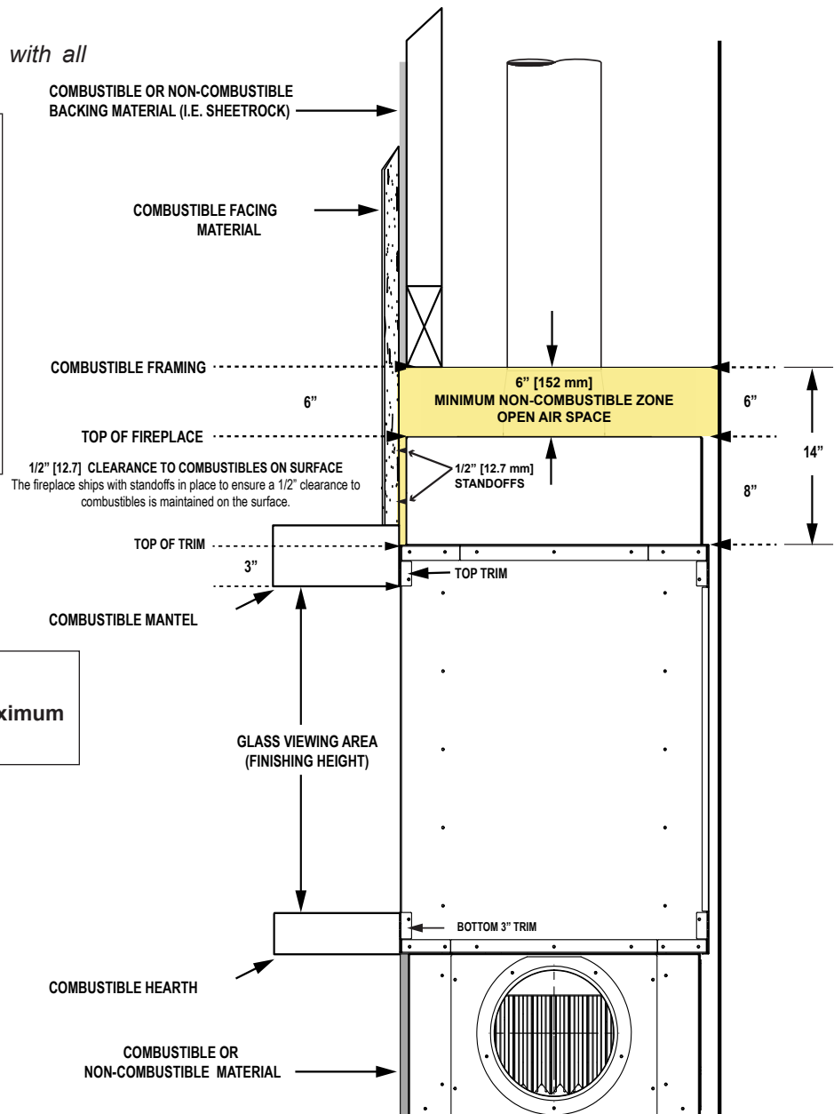
1/2" [12.7mm] Standoff
